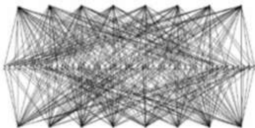
Fig. 2. Corset Hass diagram for P_{64}(T^3)
