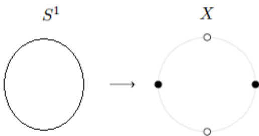
Fig. 1. Map from S^1 to P_4(S^1) ( X space) obtained by identifying equivalent points and denote the images of sets in S^1 under \Phi by x_i .
