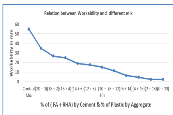
GRAPH. 3. Relation between workability and different mix.
