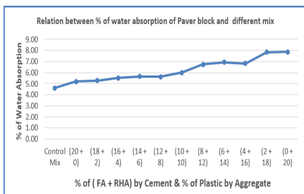
GRAPH. 4. Relation between different mix and % of water absorption of Paver block.
