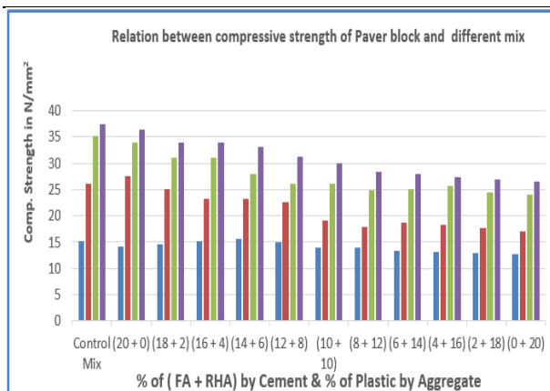
GRAPH. 2. Relation between % of Mix and compressive strength of paver block.
