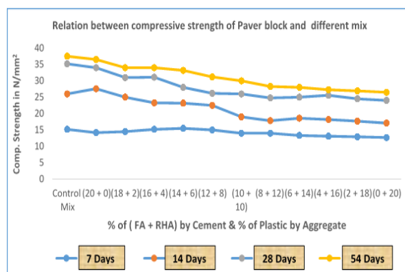
GRAPH. 1. Relation between different mix and compressive strength of paver block in days.
