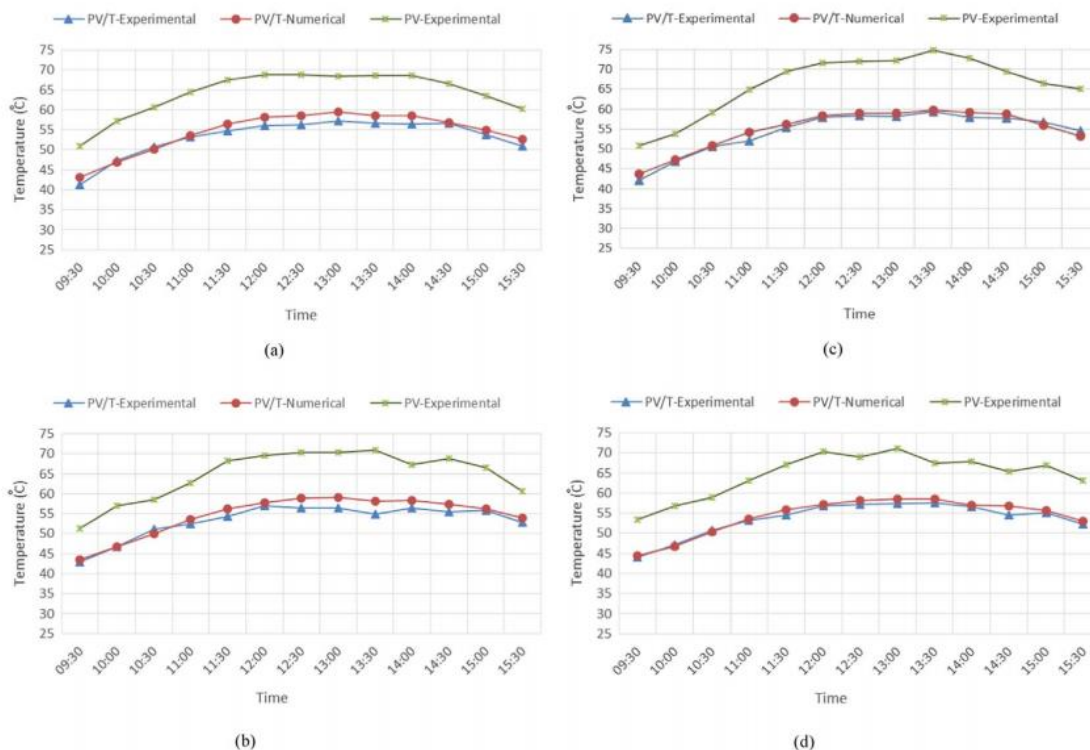
Figure 3: Measured and computed surface temperatures of the PVT system in comparison to the measured PV system values: (a) deionized water (b) TiO 2 / water nanofluid (c) ZnO/water nanofluid and (d) Al 2 O 3 /water nanofluid [25].
