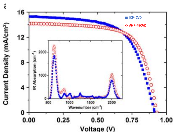
Figure 6: Current density vs voltage plots of a-Si pinsolar cells at 140 °C and infrared absorption spectra [30].
