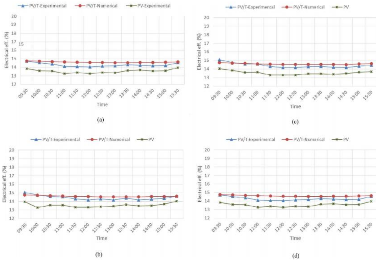
Figure 4: Experimental and numerical electrical efficiency of the different PV/T systems as compared with purely PV system: (a) Deionized water, (b) TiO 2 / water nanofluid, (c) ZnO/water nanofluid and (d) Al 2 O 3 /water nanofluid [29].
