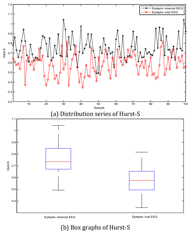
Figure 3: Distribution series and box graphs of Hurst-S between epileptic ictal and interictal EEG
