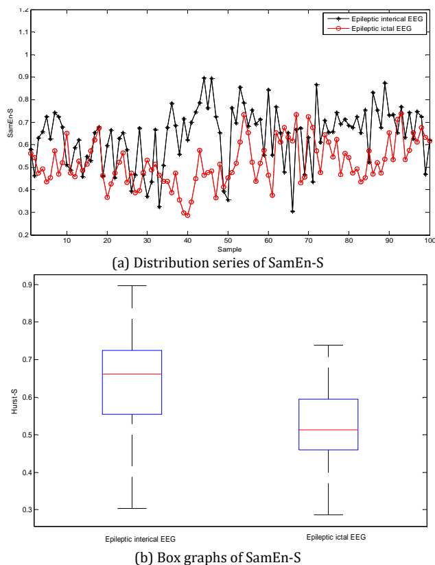
Figure 4: Distribution series and box graphs of SamEn-S between epileptic ictal and interictal EEG
