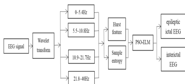
Figure 2: Flowchart of classification algorithm for epileptic EEG
