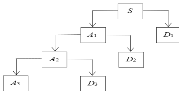
Figure 1. Scheme of 3 layer wavelet decomposition
