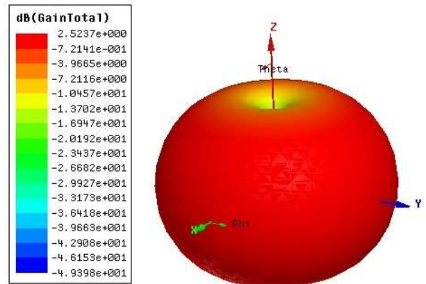
Fig.15. 3D Radiation Pattern for designed half wave dipole antenna.
