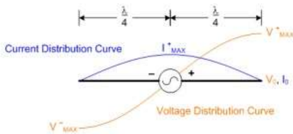
Fig. 2. Voltage and Current distribution in dipole.
