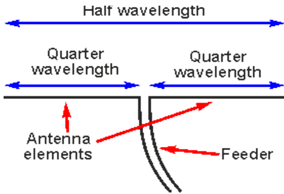
Fig.1. Half Wave dipole center feed.
