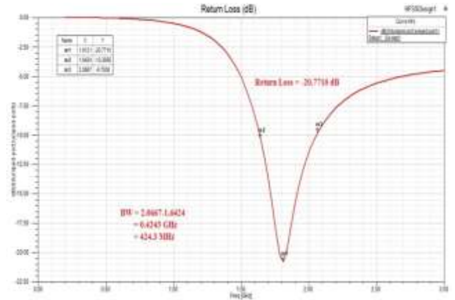
Fig.12. Return Loss curve and Bandwidth for designed half wave dipole antenna.
