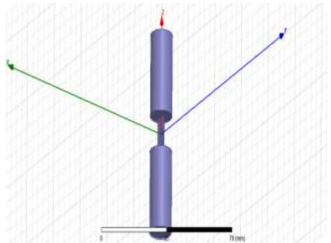
Fig.9. Designed Half Wave Dipole Antenna
