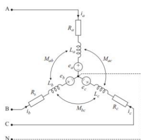
Figure 11: Equivalent circuit of three-phase BLDC motor
