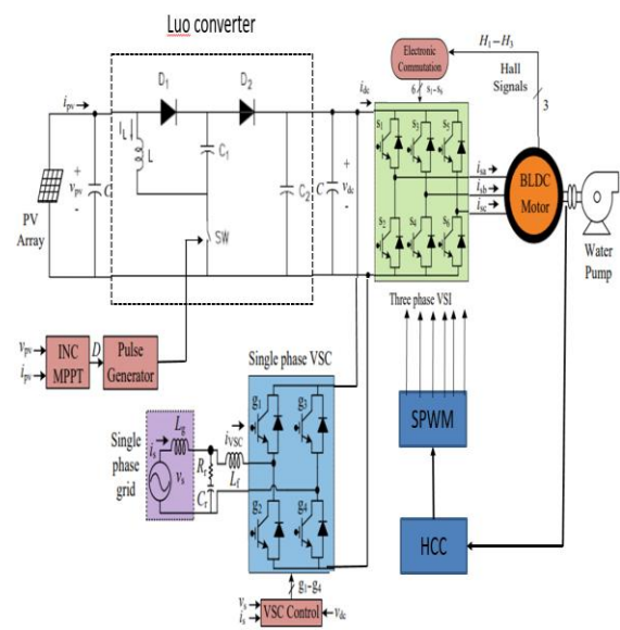
Figure 2: Power circuit of grid interactive PV array-based water pumping system using a BLDC motor drive
