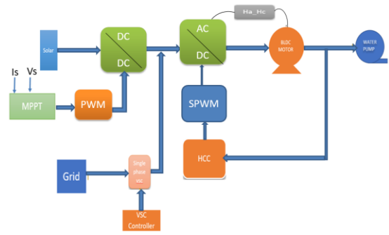
Figure.1: Block Diagram ofgrid interactive PV array-based water pumping system using a BLDC motordrive
