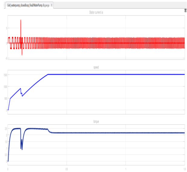
Figure 7: Stator current, speed & Torque of BLDC motor
