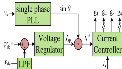
Figure 3: UVT based bi-directional power flow control of VSC
