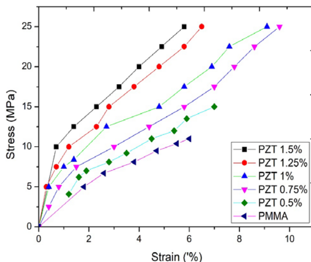
Fig. 2. Stress-strain curves of the PZT content in PMMA: PZT composite
