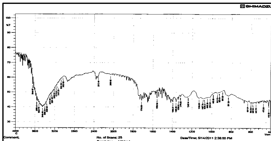
Fig. 5: FTIR spectra of carbopol 934
