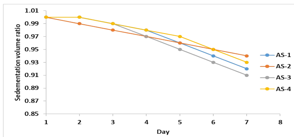
Figure 2: Sedimentation rate of AS-1, AS-2, AS-3, and AS-4
