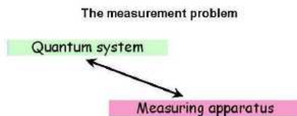
Figure 1. What is a measurement apparatus?
