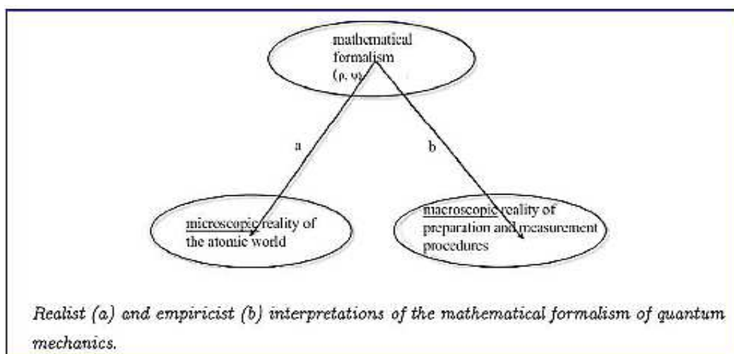
Figure 2. Realist (a) and empiricist (b) interpretations of the mathematical formalism of quantum mechanics
