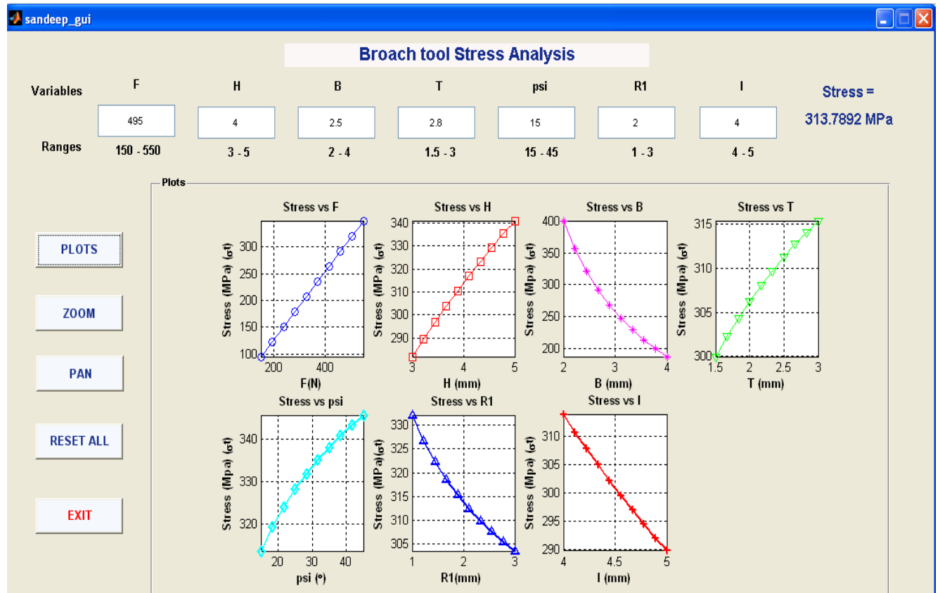
Fig. 3 GUI OF Broach tool stress analysis
