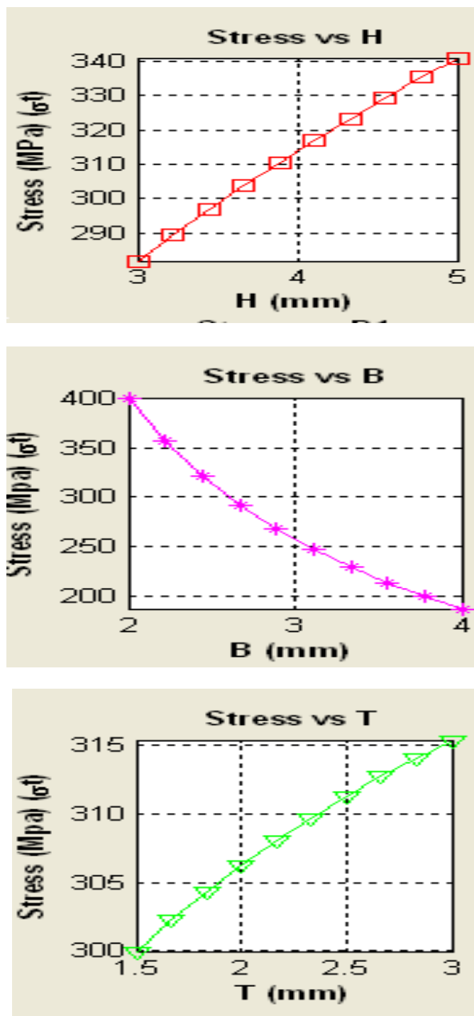
Fig. 4. Parametric variation of stress analysis
