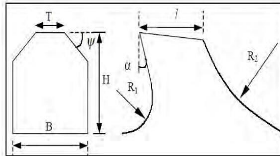
Fig. 2 General tooth profile
