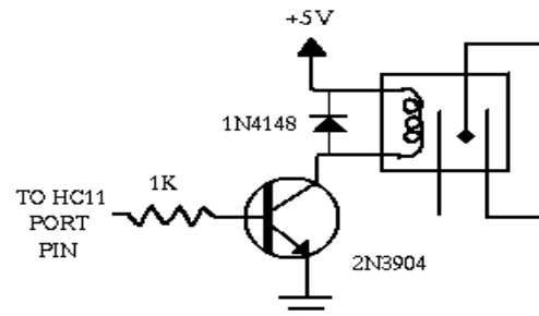
BASIC RELAY SWITCH
