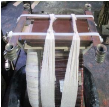
FIGURE 21(a). Resin spacer
