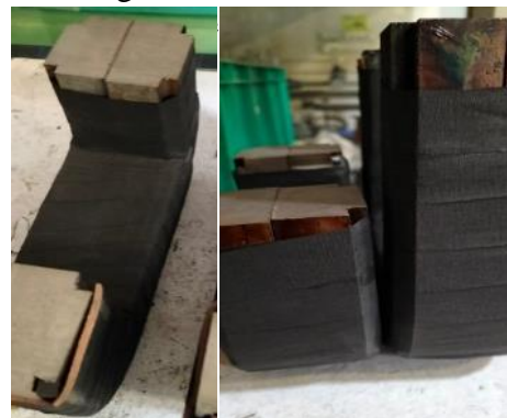
FIGURE 12(b). Padding on coil
