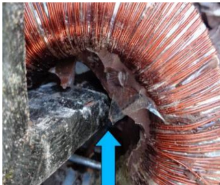
FIGURE 13(a). Open polyester between coil
