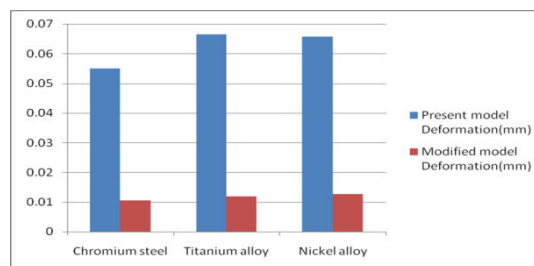
Figure: Comparisons between present and modified models of deformation
