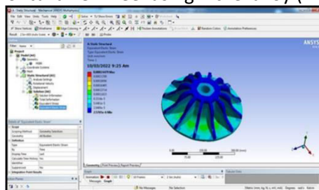
Figure: Strain of turbine wheel using Nickel alloy (modified model)
