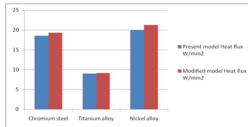
Figure: Comparison between present and modified model of heat flux
