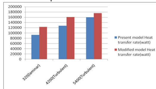
Figure: Comparison between present and modified models of heat transfer rate By observing CFD analysis results, the heat transfer rate and heat transfer coefficient are more for modified model compared to present model, mass flow rate is less for modified model compared to present model. So, the modified model is better than present model.
