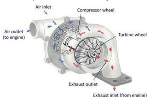
Figure 1.1 Turbo Charger
