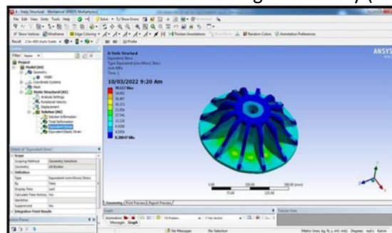
Figure: Stress of turbine wheel using nickel alloy (modified model)
