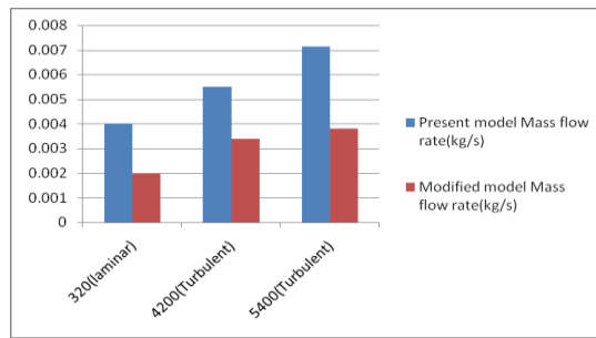
Figure: Comparison between present and modified models of mass flow rate
