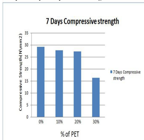
Graph: 7 days compressive strength
