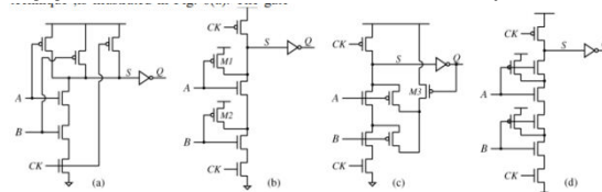
Fig6. Constructing complementary PFET network (2-input AND gate). (a) Complementary p-network technique . (b) CMOS inverter technique .(c) Gated CMOS inverter technique [20]. (d) Triple transistor technique .
