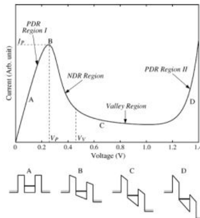
Fig16. Typical I-V characteristic of resonant tunneling diodes and schematic band diagrams The narrow well are discretized due to the quantization effect. Quantum tunneling, also known as resonant tunneling, occurs when the applied voltage across the diode is aligned to one of the discrete energy levels in the well resulting in sharp current peak [28]. Schematic band diagrams at four different voltage values across the diode are illustrated in Fig. 16. Also shown in the figure is the I - V characteristic of a typical RTD. It consists of a positive differential resistance (PDR) region, a negative differential resistance region, a valley region, and a second PDR region. RTD operates in PDR Region I. The gate enters the evaluate phase when CK switches high. The RTD stays in the PDR Region I until the input voltage to the pull-down network is high enough such that the discharge current exceeds I_p , the peak current of the RTD. After this point, the gate starts to accelerate in switching because the combined effect of increasing discharge current and the decrease in the pull-up current through the RTD. After the dynamic node S drops to a certain low voltage value, the PFET in the keeper is switched off allowing the dynamic node to fully reach the ground voltage. In all, it can be observed that dynamic logic circuits designed using the proposed method maintain the following benefits that conventional domino logic gates possess:
