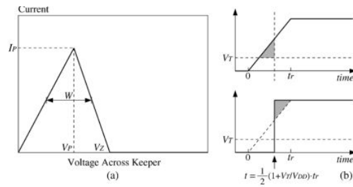
Fig17. Assumption for simple analysis. (a) Piecewise linear NDR keeper I-V characteristic. (b) Input voltage waveform (top: saturated ramp waveform; bottom: equivalent step waveform). keeper, the keeper operates in PDR region. The voltage drop at the dynamic node S is less than or equals to and the output of the gate driver remains low. However, when the input noise voltage is large so that the discharge current of the n-network is greater than , the keeper operating point moves into the NDR region. The current supplied by the keeper reduces steeply and the voltage at the dynamic node S quickly drops resulting in a low-to-high switching of the gate driver. Overall, the maximum input noise level that the dynamic gate can withstand is the voltage that causes the voltage level at the dynamic node S to drop to .
