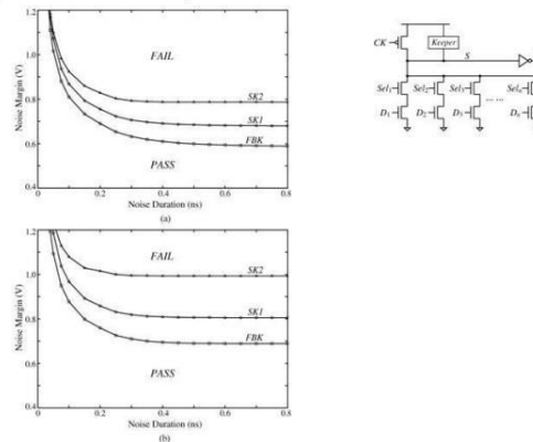
Fig21. Dynamic noise rejection curves. (a) When delay overhead is 10%. (a)When delay overhead is 20%.
