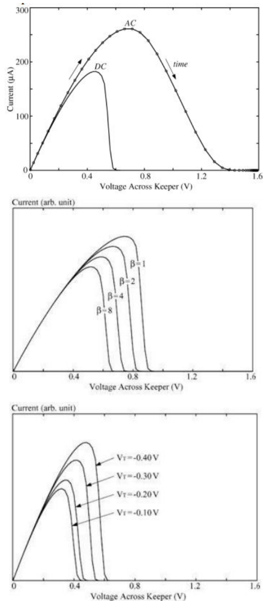
Fig10. Impacts of transistor sizing and threshold voltage on I-V characteristic. (a) With respect to beta ratio. ( V = 0:40V .) (b) With respect to threshold voltage ( = 4:0 ).
