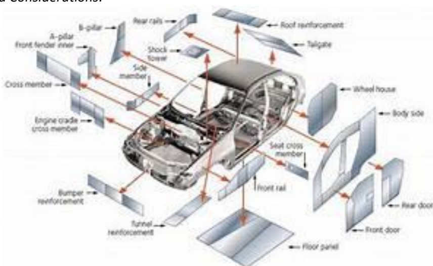
Fig 2. Lightweight vehicle Design
