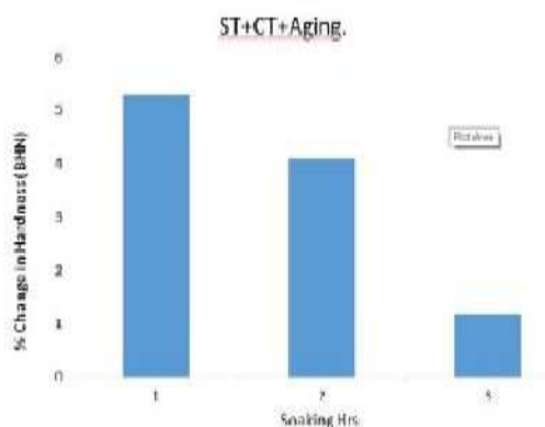
Fig7.ST+CT+Aging effect on hardness
