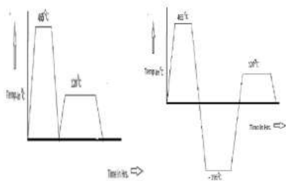
Fig. 2. T6 Treatment Fig.3.Solutionizing + Cry. Treatment + Aging
