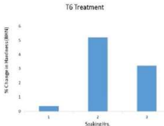
Fig.4.T6-Effect on Hardness
