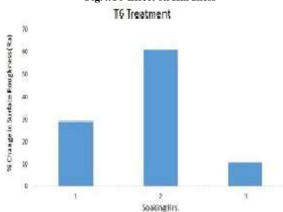
Fig.5.T6-Effect on Surface Roughness
