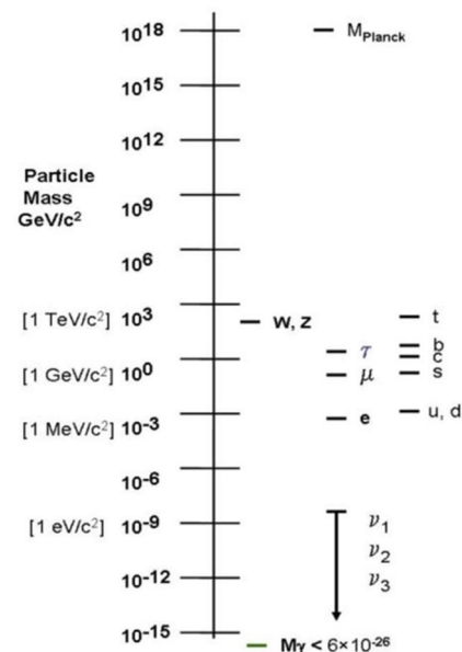
Figure 1. Spectrum of the elementary particles. Brain photons=quantons have energy 10^{-15} eV.
