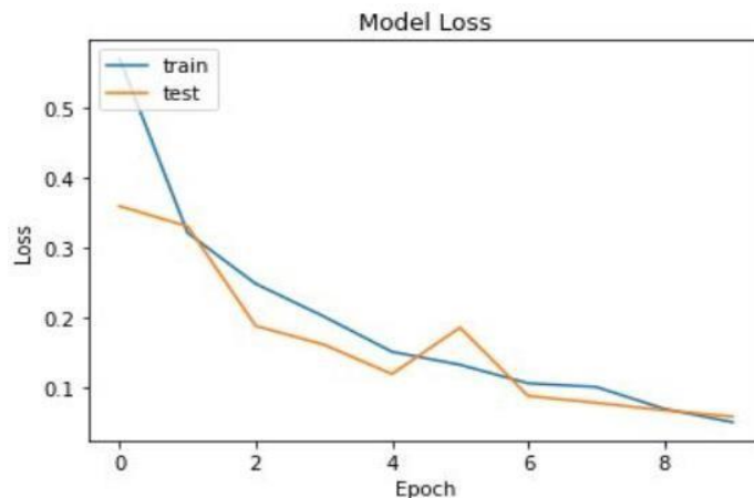
Figure 4. Train & Test loss vs. Number of Epochs
