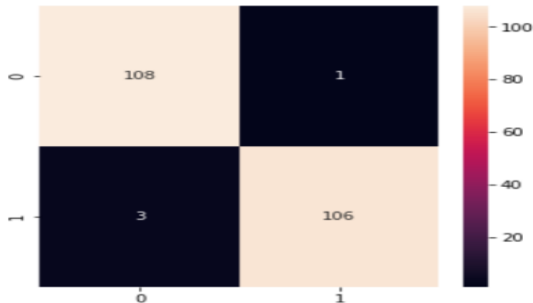
Figure 6. Classification report
