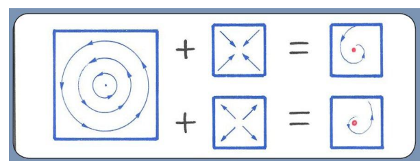
Figure 1. An unstable center can be perturbed into a point attractor or point repeller. Taken from Abraham and Shaw with permission (2005, Fig. 12.1.8, p. 368)
