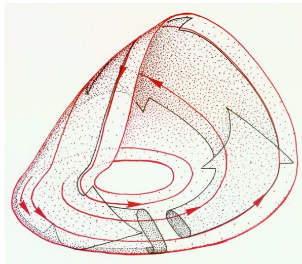
Figure 5. Rössler's Chaotic Attractor, showing divergence. Image from Abraham and Abraham with permission (2010, p. 16).
