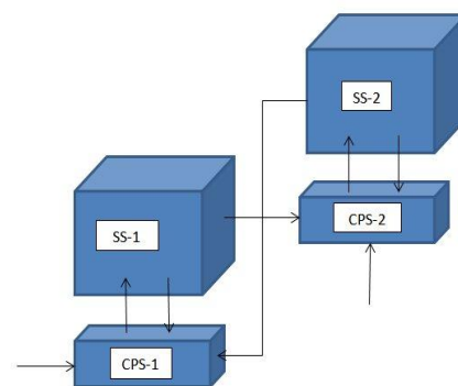
Figure 4. Small Network. SS = State Space, CPS = Control-Parameter Space. Adapted from Abraham and Abraham, 2010 with permission.
