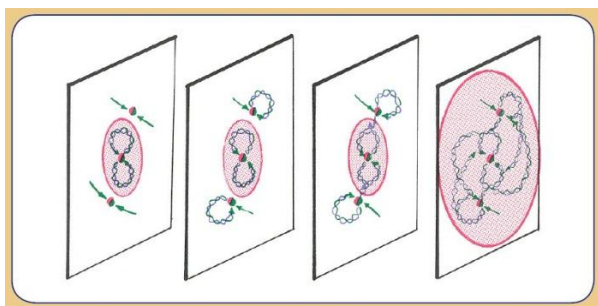
Figure 2. Portraits of Ueda’s Explosive Bifurcation, an example of a chaos-to-chaos bifurcation. Taken from Abraham and Shaw with permission (2005, Fig. 21.4.9, p. 609).
