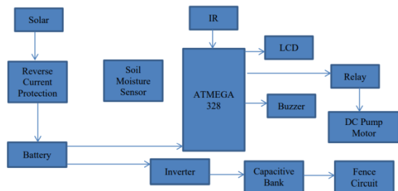
Fig. 1: Block Diagram of Fence Circuit and Automatic Irrigation System.
